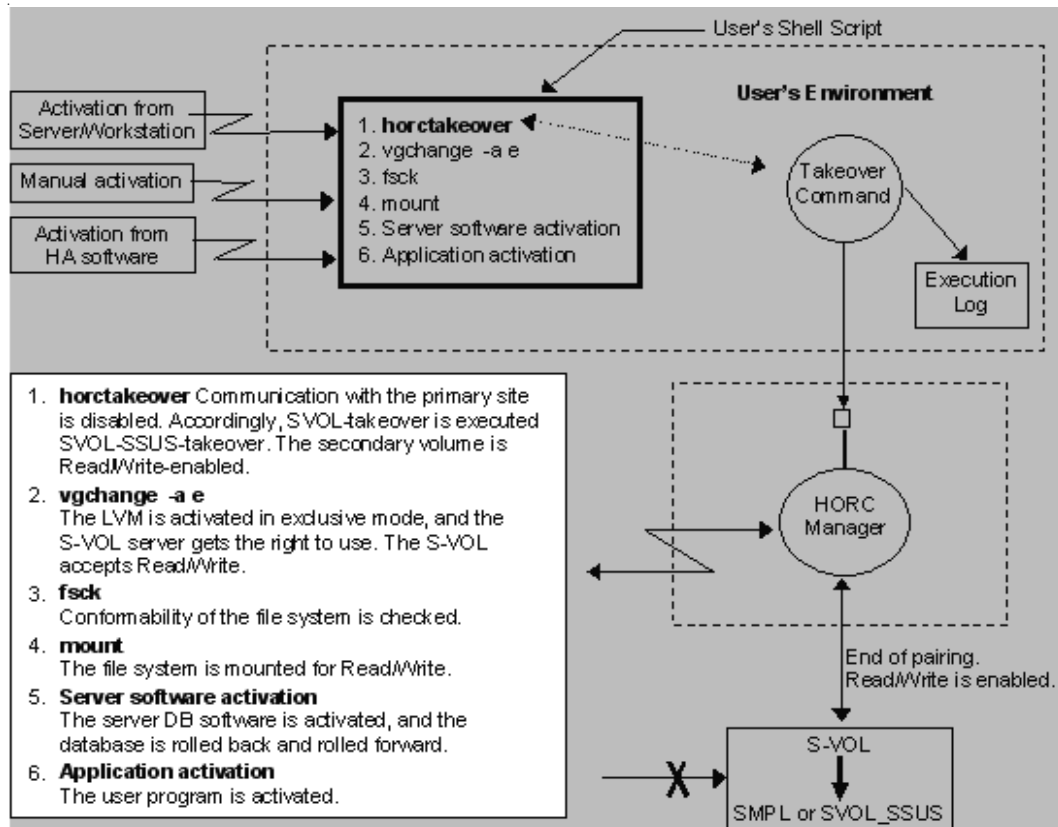
Figure 1-37: TrueCopy or TCE Takeover Example (Windows System)
