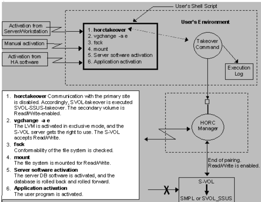
Figure 1-36: TrueCopy or TCE Takeover Example (UNIX System)
